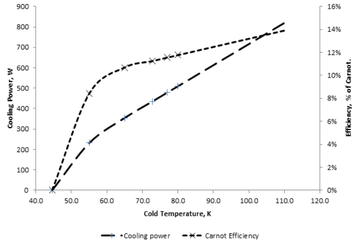
PTC330 Cooling Curve
